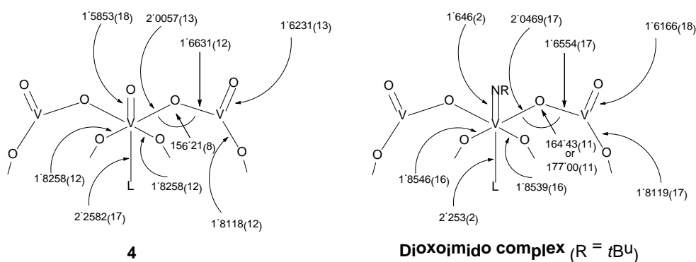
Scheme 2. Comparison of selected bond lengths of 4 versus the dioxoimido complex \{[(\text{VN}t\text{Bu})(\text{THF})_{0.39}(\text{OtBu})_{0.61}][(\text{VO})(\mu\text{-O})_2\text{L}^6][t\text{BuNH}_3]\} . [4a]
