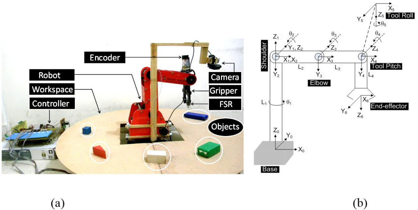
Figure 3. (a) AUTAREP – An open source pseudo-industrial framework (Ajwad et al., 2016); (b) Kinematic representation (Ajwad et al., 2015a).
