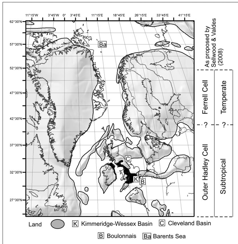
Figure 1. Paleogeography of NW Europe for the Kimmeridgian Stage (provided by Getech Group plc) including the sea level highstand line and the present-day countries rotated to their palaeopositions. The distribution of the Hadley cell and associated climate belts is based on previous work [Sellwood and Valdes, 2008], which we revise in this paper.
