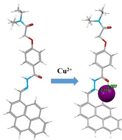
Fig. 6 Geometry-optimized (PBE0/LANL2DZ) structures of L1 with complex Cu 2+ ion. Left : The free ligand L1 (Ellipsoid); Right : Ligand L1 complex with Cu 2+ ion (Ellipsoid). Colour code: carbon = dark grey and oxygen atom = red, nitrogen = blue and Cu 2+ = purple.
