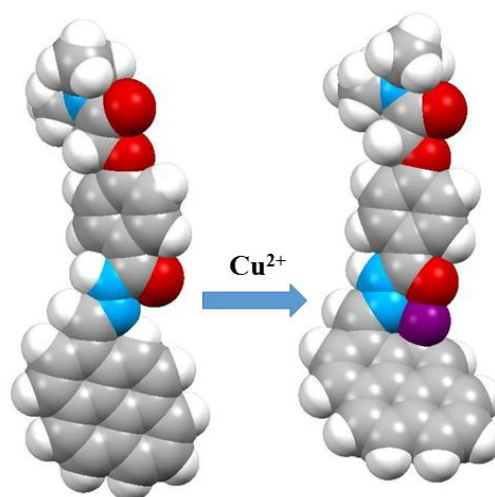
Fig. 8 Geometry-optimized (PBE0/LANL2DZ) structures (Space fill) of L1 and as its \text{Cu}^{2+} complex ion. Left : The free ligand L1 ; Right : 1:1 \text{L1}\rightarrow\text{Cu}^{2+} complex. Colour code: carbon = drack grey and oxygen atom = red, nitrogen = blue and \text{Cu}^{2+} = purple.
