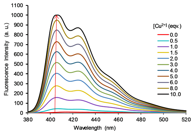
Fig. 4 Fluorescence spectra of ligand L1 (1.0 \mu\text{M} ) upon addition of increasing concentration of \text{Cu}^{2+} ions (0–10 equiv.) measured in \text{CH}_3\text{CN}/\text{CH}_2\text{Cl}_2 (1000:1, v/v). \lambda_{\text{ex}} = 367 nm.
