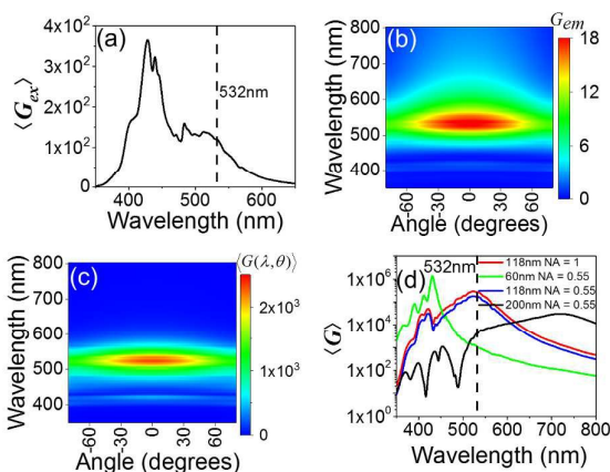
Fig. 3: (a) Calculated near field enhancement factor ( G_{ex} ) for a 5 nm nano-gap formed between a 118 nm silver particle and a 100 nm extended silver film. (b) Calculated emission enhancement factor G_{em} for the same nano-gap. (c) Calculated Raman enhancement ( G(\lambda, \theta) ) for the same nano-gap. (d) Calculated Raman enhancement ( G(\lambda) ) for NA = 0.55, for a 5 nm nano-gap of different particle size 60 nm, 118 nm and 200 nm. For comparison, \langle G(\lambda) \rangle integrated over NA = 1 for the 118 nm particle nano-gap is also presented.
