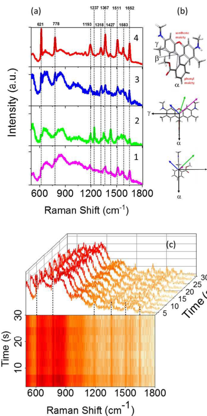
Fig. 5: (a) Spectra 1-3 show three typical single molecule Rhodamine 6G SERS spectra recorded from three different 5 nm nano-gaps formed between a 118 nm silver particle and a 100 nm extended silver film. For comparison we plot in panel 4 a high concentration ( 5 \times 10^{-5} M) SERS spectrum of Rh6G. (b) Top part: Rhodamine 6G molecule with main moieties indicated. Bottom part: the projection of the nano-gap field on molecules 1, 2 and 3 in \alpha - \gamma and \alpha - \beta planes. (c) Time dependent single molecule SERS spectra (accumulation time 3 s, total time 30 s).
