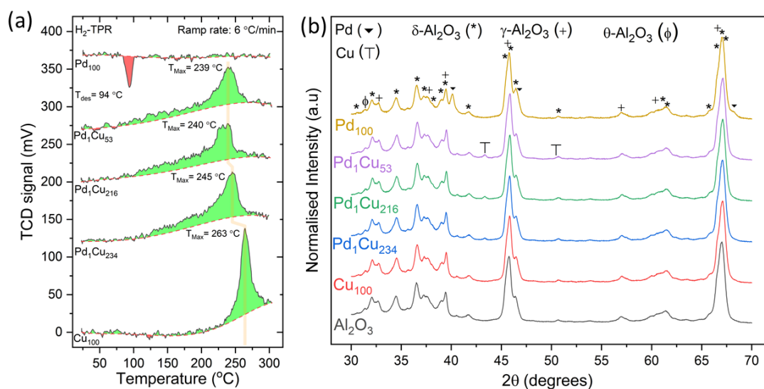
Fig. 1 (a) H_2 Temperature programmed reduction of Cu, PdCu and Pd catalysts. Gas composition was 5% H_2 /95% N_2 v/v at 40 ml min^{-1} with a heating rate of approximately 6 ^{\circ}C\ min^{-1} . (b) XRD diffractograms of reduced ex situ Pd, Cu and PdCu species supported on Al_2O_3 catalysts and the bare support.
