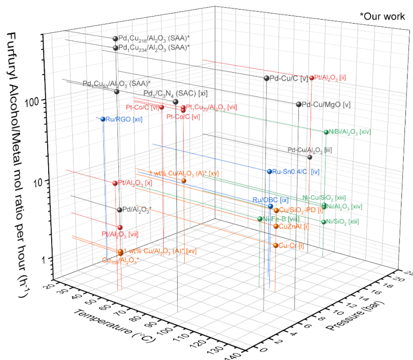
Fig. 9 Furfuryl alcohol/metal mole ratio per hour of catalysts from this work and various catalysts found in the literature under low to moderate conditions ( <140\text{ }^{\circ}\text{C} and <20\text{ bar} ). Square bracketed Roman numerals [i], [ii], [iii], [iv], [v], [vi], [vii], [viii], [ix], [x], [xi], [xii], [xiii], [xiv] and [xv] represent references [91], [92], [14], [20], [90], [15], [6], [93], [94], [2], [89], [95], [96], [97] and [22], respectively. Log 10 scale is used for the furfuryl alcohol/metal ratio per hour z axis and the colour of the spheres represents which metal is used for the calculation. Pd, Pt, Ru, Ni and Cu represent sphere colours dark grey, red, blue, green, and orange, respectively.
