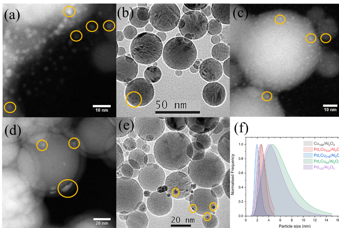
Fig. 2 STEM/TEM images of (a) Cu 100 /Al 2 O 3 , (b) Pd 1 Cu 234 /Al 2 O 3 , (c) Pd 1 Cu 216 /Al 2 O 3 , (d) Pd 1 Cu 53 /Al 2 O 3 , (e) Pd 100 /Al 2 O 3 , and (f) lognormal STEM/TEM size distributions for the catalysts reduced ex-situ at 300 °C for 0.5 h under flowing H 2 .
