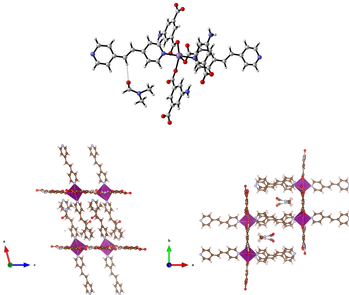
Fig. 8 Top: Diagram of 7-6DMF showing the coordination environment around the \text{Mn}^{2+} nodes. The weak C–H...O hydrogen bond between the dipyrindyl linker and the DMF molecule is represented by a dashed line. Bottom: Diagram of the extended structure of 7-6DMF showing the weakly hydrogen-bonded DMF molecules situated inside the pores ( b and c axes). Carbon, nitrogen, oxygen, and manganese atoms are coloured brown, blue, red, and rose red, respectively.
