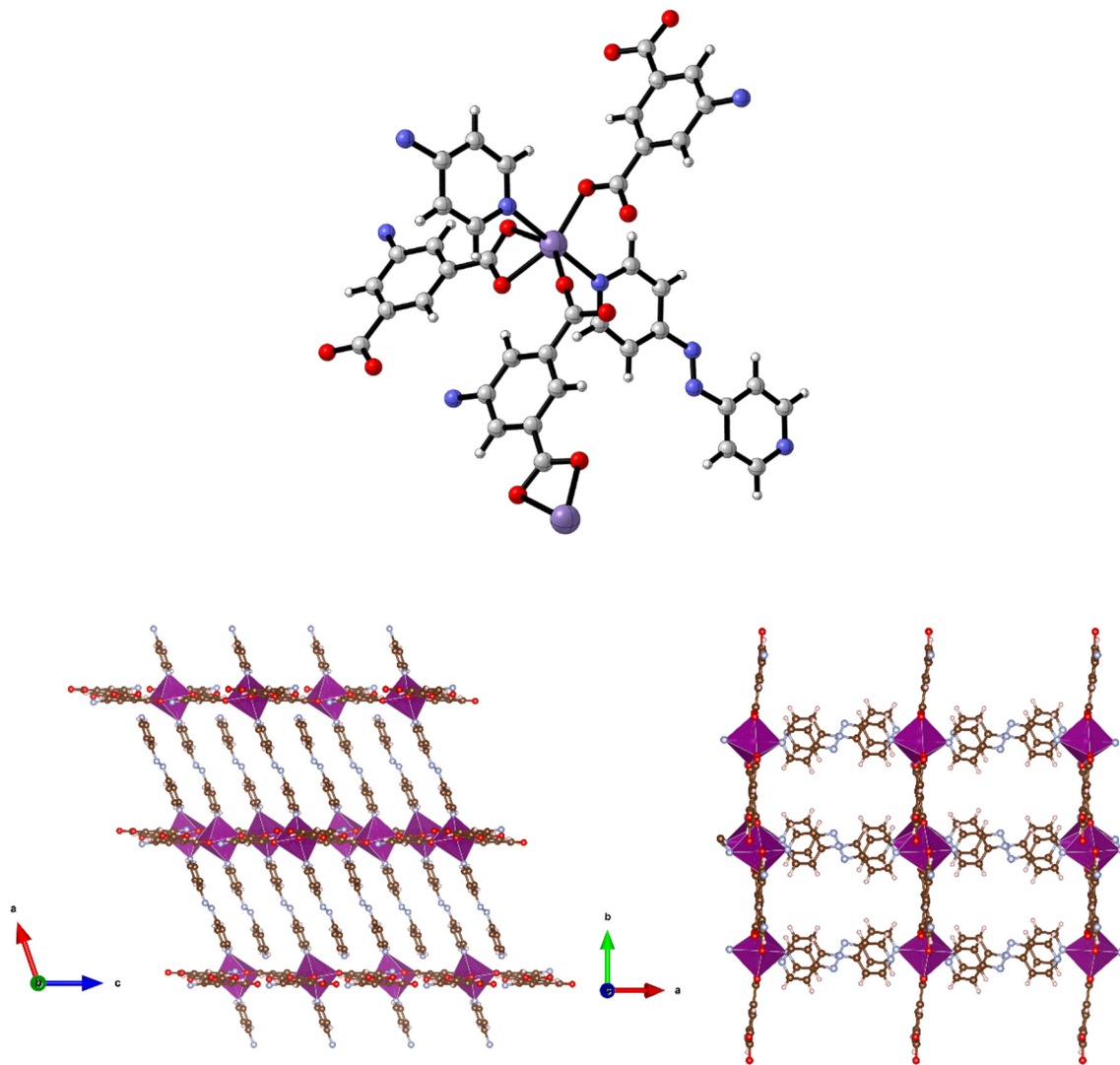
Fig. 9 Top: The metal coordination environment in [\text{Mn}(5\text{-AIP})(4,4'\text{-azopy})] \cdot 8 \cdot 2.5\text{DMF} . Bottom: Diagram of the extended structure of 8 \cdot 2.5\text{DMF} (parallel to the b (left) and c (right) axes).
