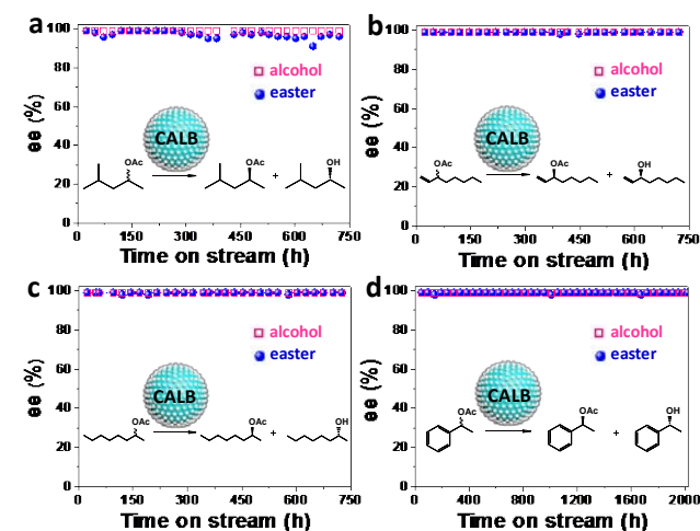
Figure 8. CALB enzyme-catalyzed hydrolysis kinetic resolution of racemic acetates using the FPE method (the column is 3.6 cm in diameter). The Pickering emulsions were formulated with 40 mL aqueous enzyme ( 0.1 \text{ mg mL}^{-1} , 0.5 \text{ M Na}_2\text{HPO}_4 ), 20 mL n -octane and 1.2 g
