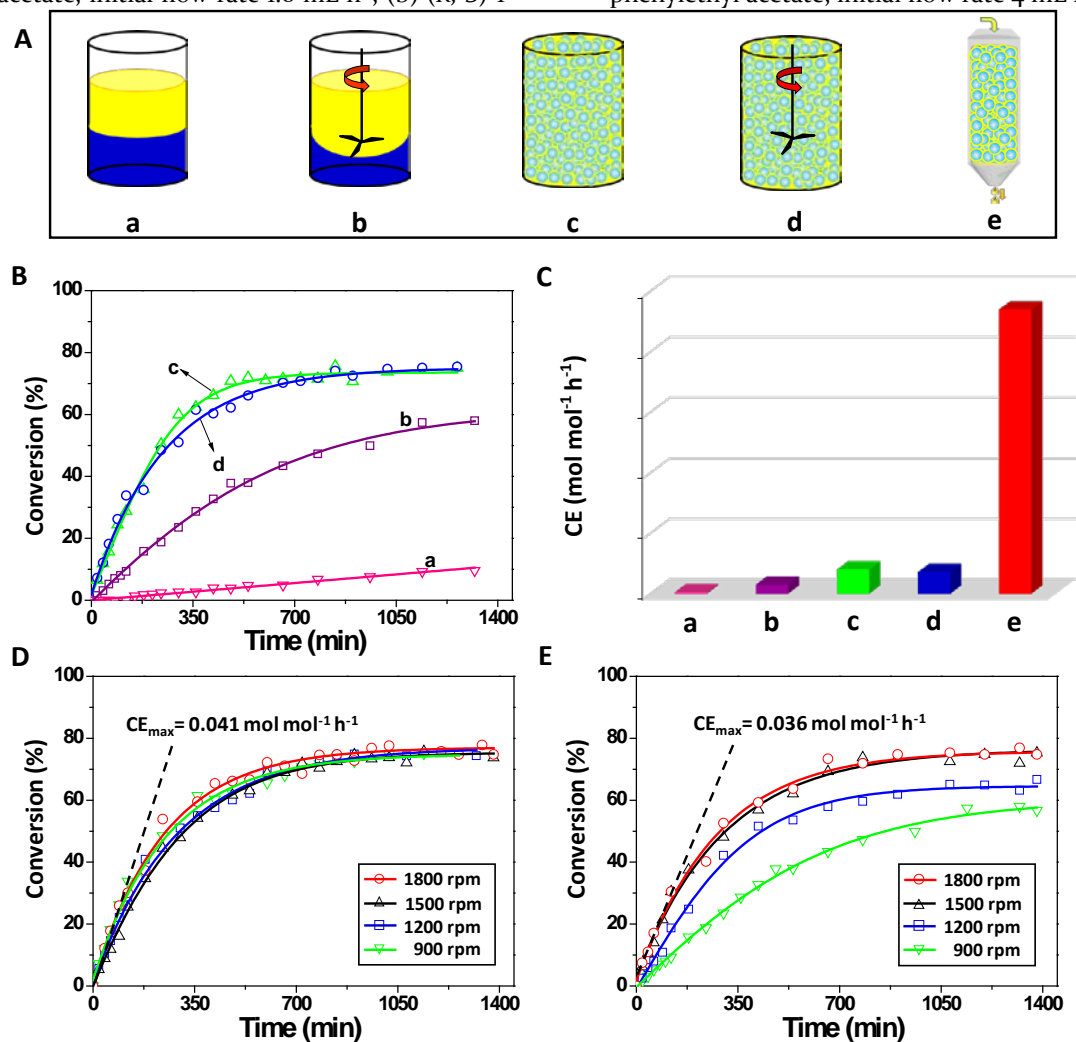
Figure 9. Comparison of the H 2 SO 4 -catalyzed addition of n -octanol with 3, 4-dihydro-2 H -pyran using the existing biphasic batch reactions and using the FPE reaction. (A) Cartoon representation of various reaction systems. a - agitation-free biphasic reaction, b - biphasic reaction with agitation speed of 900 rpm, c - agitation-free Pickering emulsion reaction, d - Pickering emulsion reaction with agitation speed of 900 rpm, e - FPE reaction. Batch reaction conditions: 8 mL aqueous H 2 SO 4 (0.5 M), 4 mL reactant solution in toluene (0.25 M), 50 °C, 0.16 g emulsifier if needed. The reaction conditions of the FPE system are the same as in Figure 5a except the flow rate = 2.5 mL h -1 . (B) Kinetic reaction profile with time for the batch reactions. (C) Catalysis efficiency (CE) of the batch reactions over 550 min and the FPE reaction after the conversion levelled off. (D) Pickering emulsion systems at different agitation speeds. The maximum catalysis efficiency (CE max ) is given under the mass transport limitation-free conditions calculated at the beginning of reaction. (E) Conventional batch biphasic systems at different agitation speeds.
