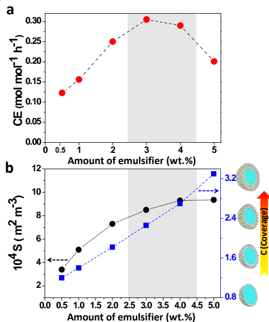
Figure 6. Relationship between the FPE catalysis efficiency of the addition of n -octanol with 3, 4-dihydro-2H-pyran and interface properties. The flow rate was maintained at 2.5 mL \text{h}^{-1} . Other reaction conditions are the same as in Figure 5a. (a) Catalysis efficiency (CE) vs emulsifier amount. CE is defined as the moles of converted reactants per mole of catalyst per h (mol mol -1 h -1 ), calculated after the conversion levelled off (above 5 h). (b) Oil-water interfacial area S and coverage of interface by particles C vs emulsifier amount.
