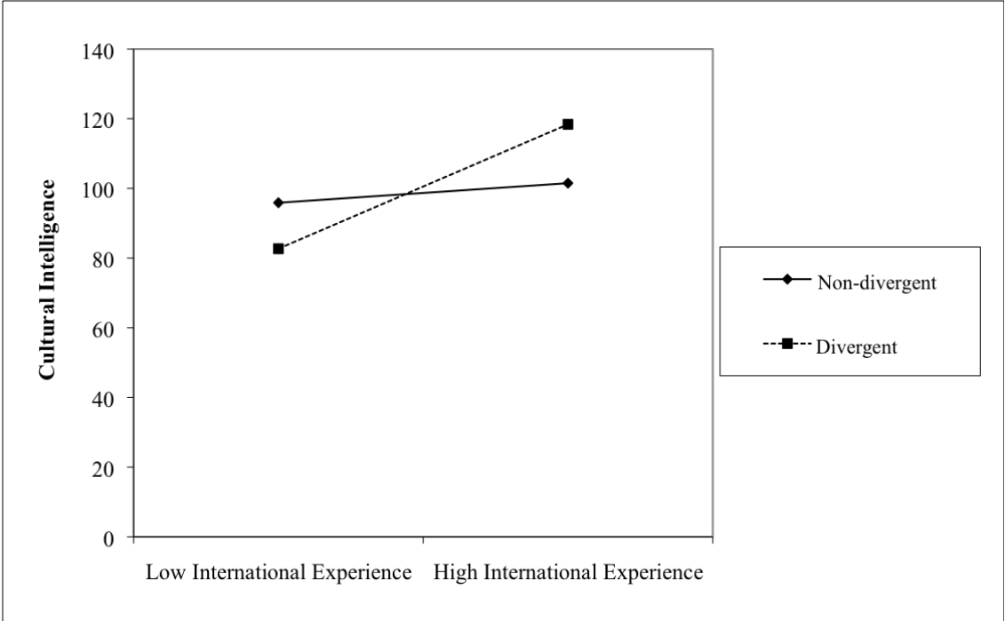
Figure 3. Interaction Effect
